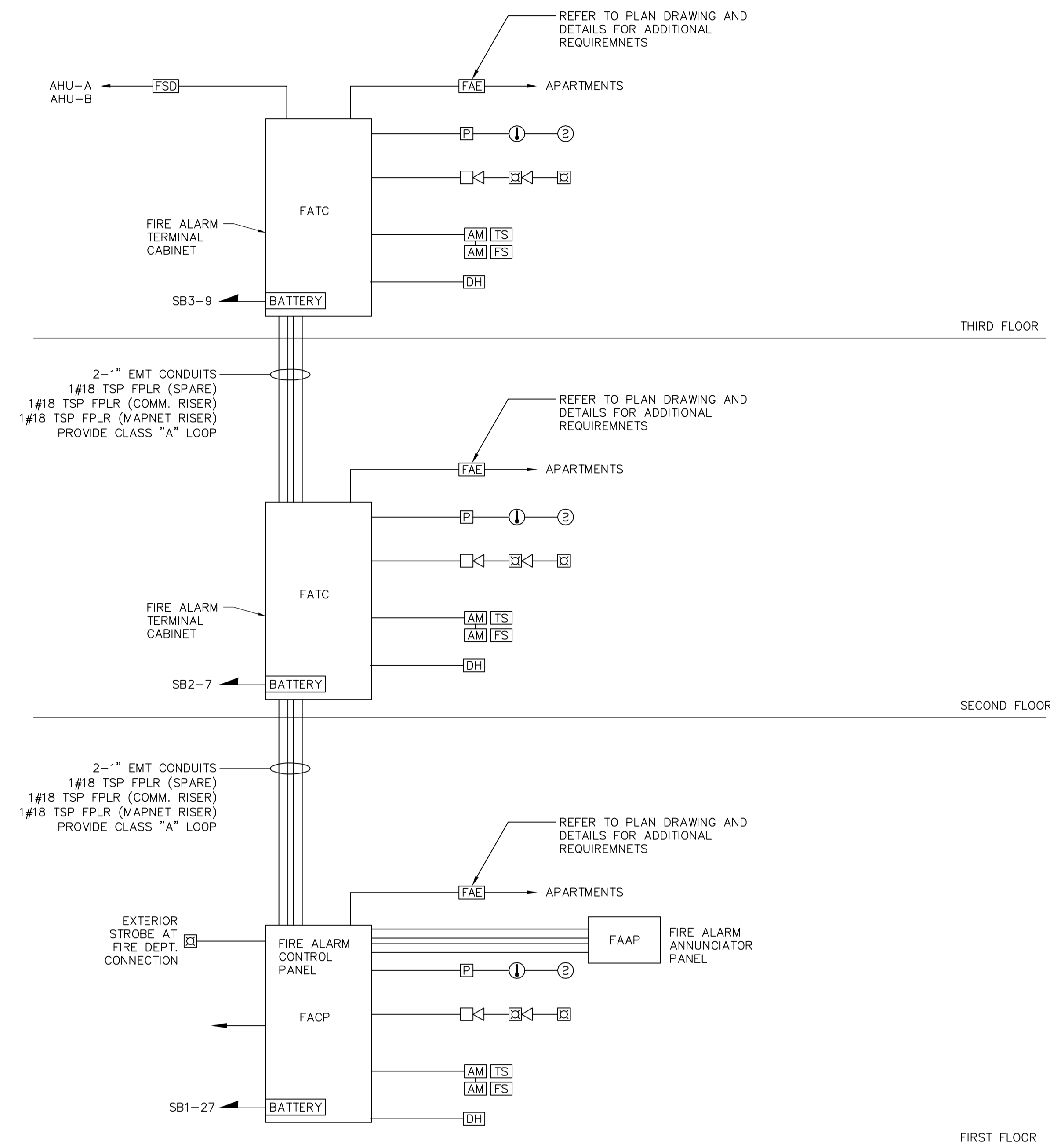
(A) FIRE ALARM SYSTEM RISER DIAGRAM SCALE: NONE
