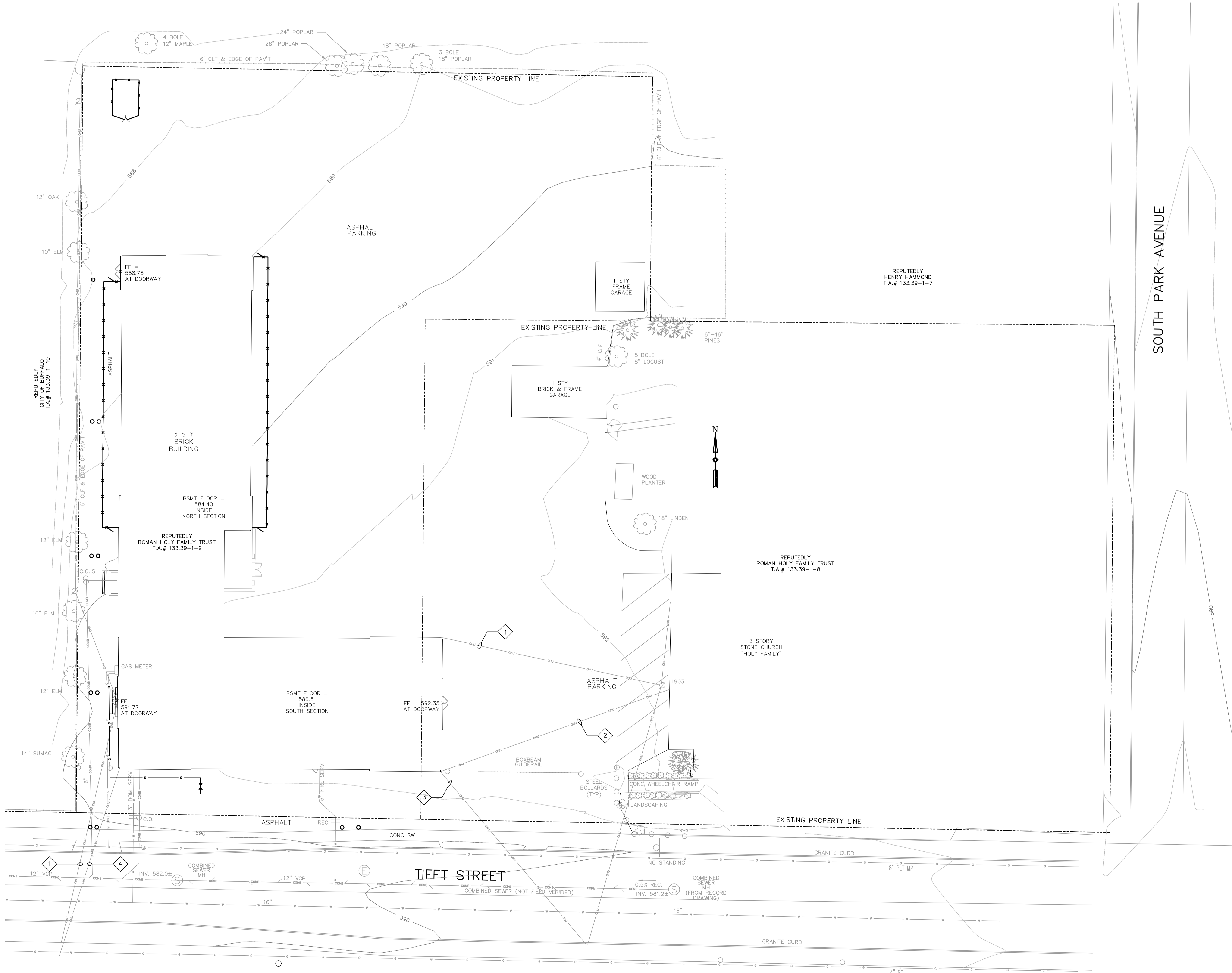
(A) ELECTRICAL SITE DEMOLITION PLAN SCALE: 1"=20'-0"
