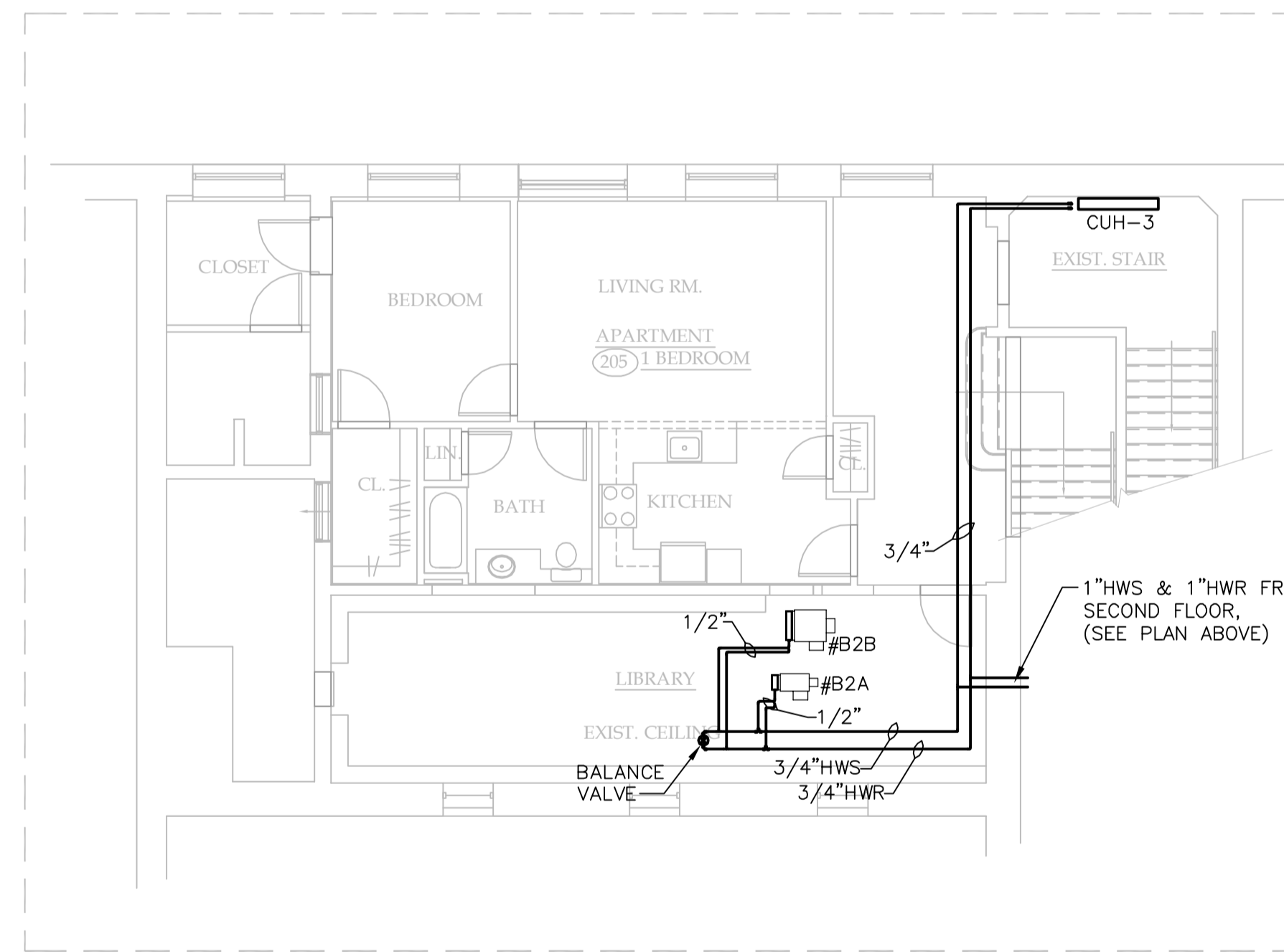
(B) HVAC PIPING SECOND FLOOR PLAN - BRIDGE SCALE: 1/8" = 1'-0"
